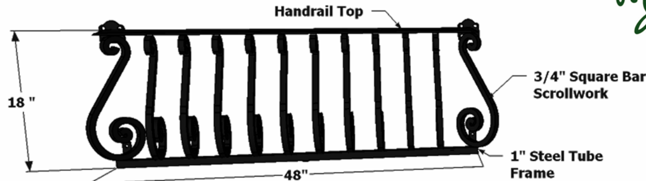
Front View
